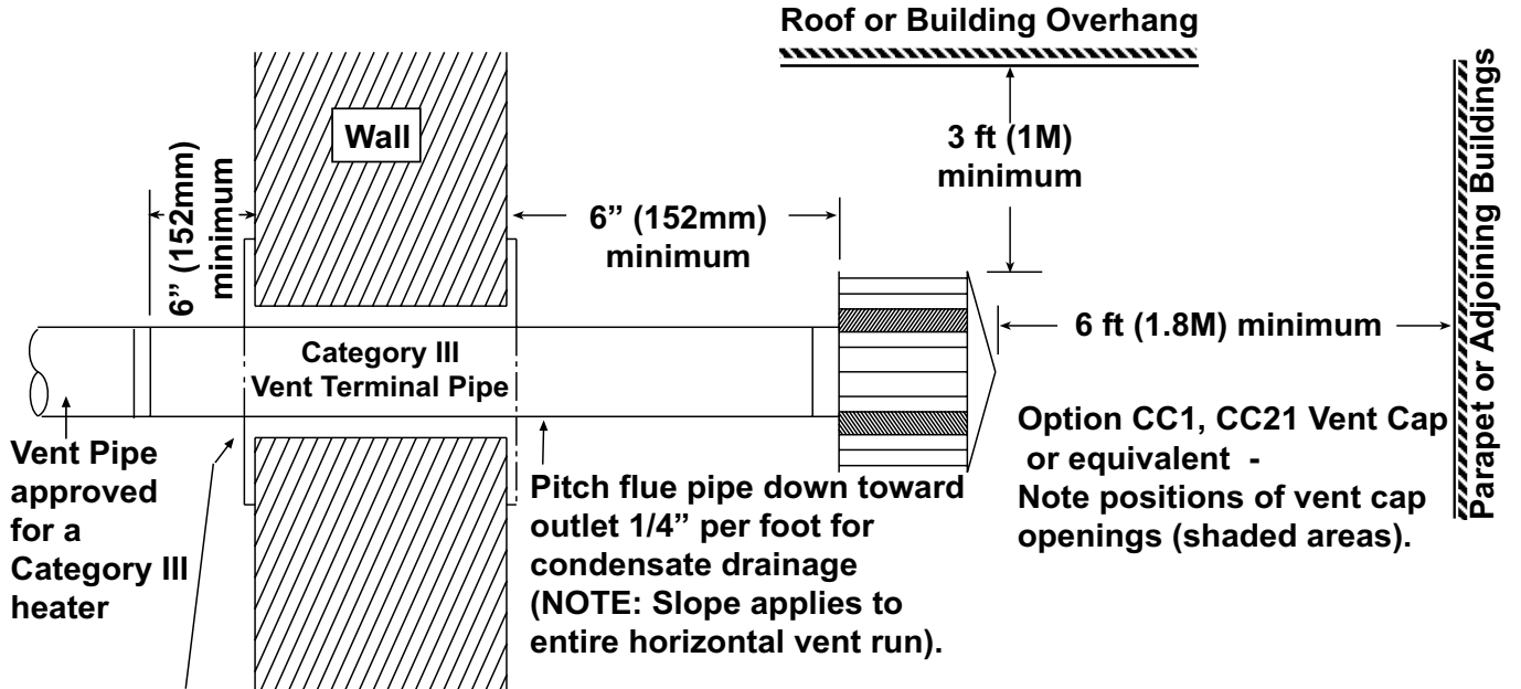
FIGURE 1 - Horizontal Vent Terminal - Residential Installation
